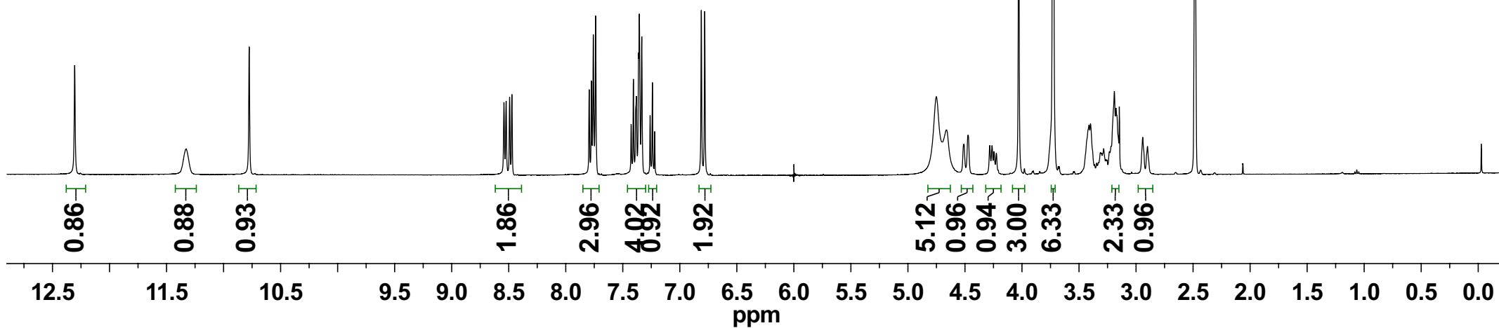
Elacridar hydrochloride 400MHz ^1\text{H} NMR \text{DMSO-}d_6
