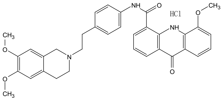
Elacridar hydrochloride 400MHz ^1\text{H} NMR \text{DMSO-}d_6
