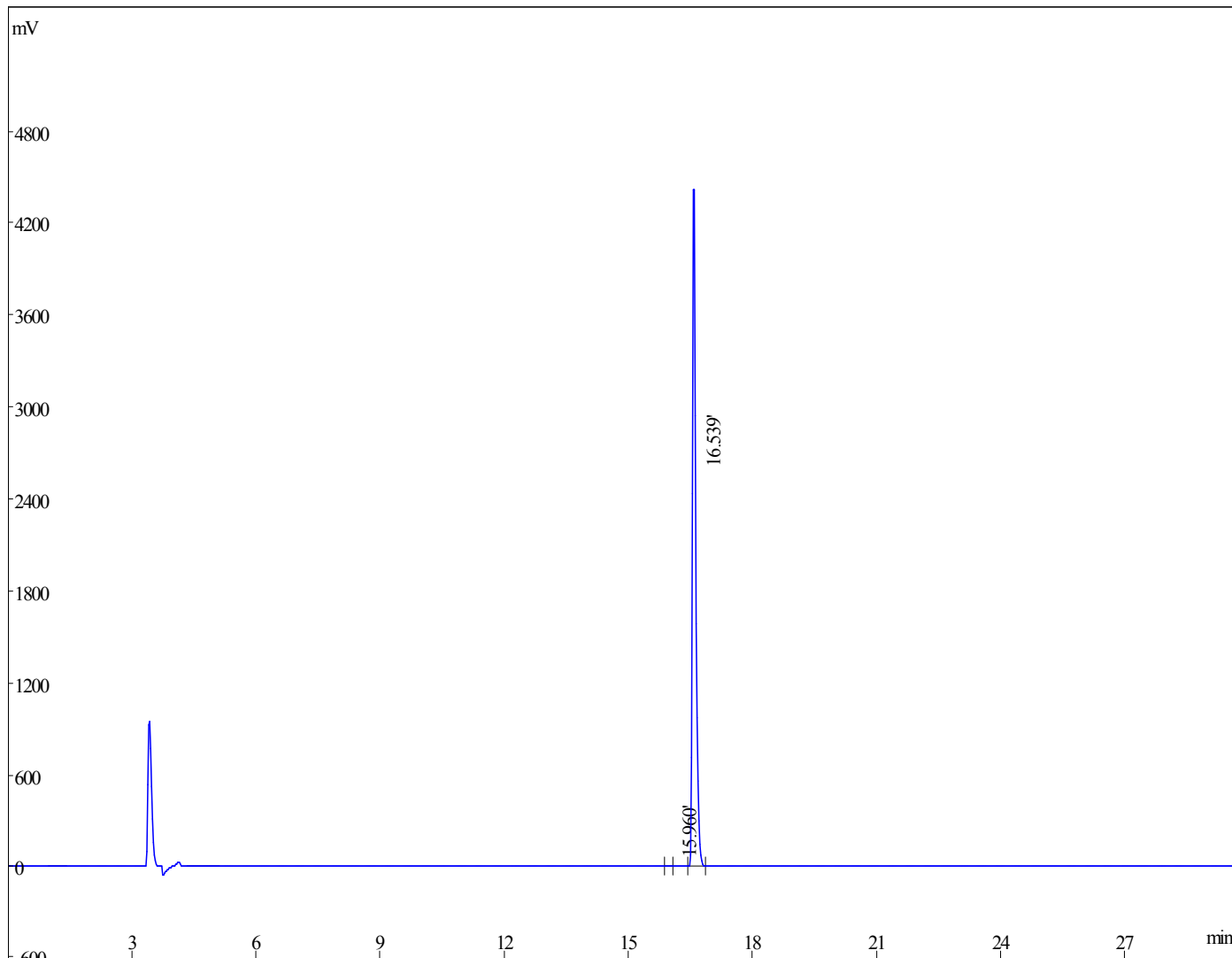
Chromatogram
